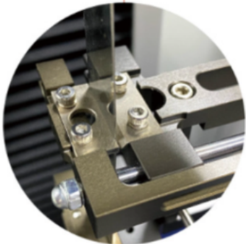
Clamp for Flat Specimen
